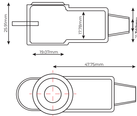
TCMR & TCMB Medium Terminal Cover
