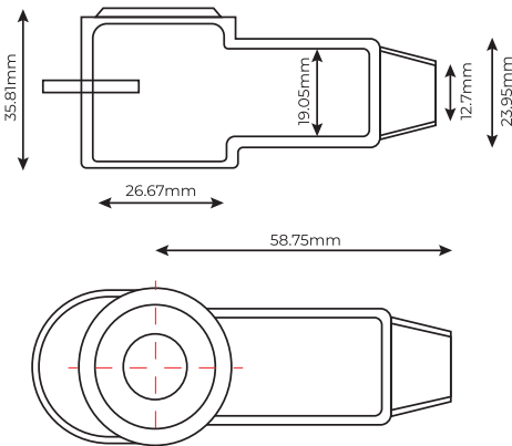
TCLR & TCLB Large Terminal Cover
