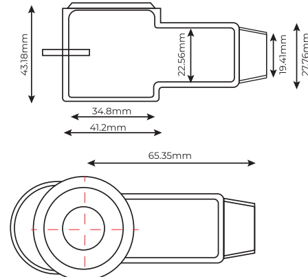
TCXLR & TCXLB Extra Large Terminal Cover
