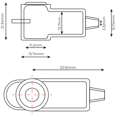
TCSR & TCSB Small Terminal Cover
