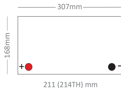
Terminal Style M8 Insert
