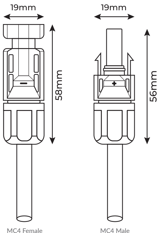
MC4 Solar Connectors
