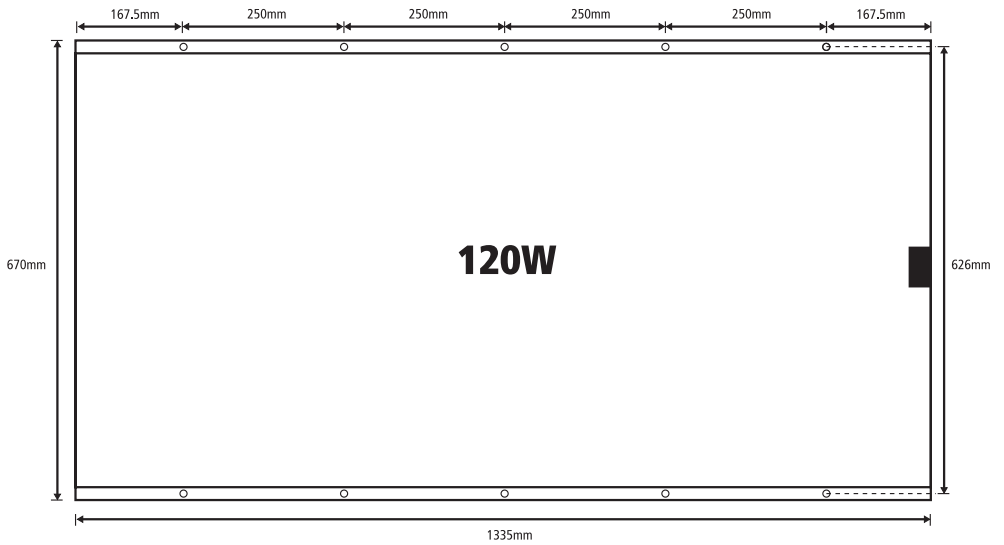
FIXING HOLE DIMENSIONS (NOT DRAWN TO SCALE)
