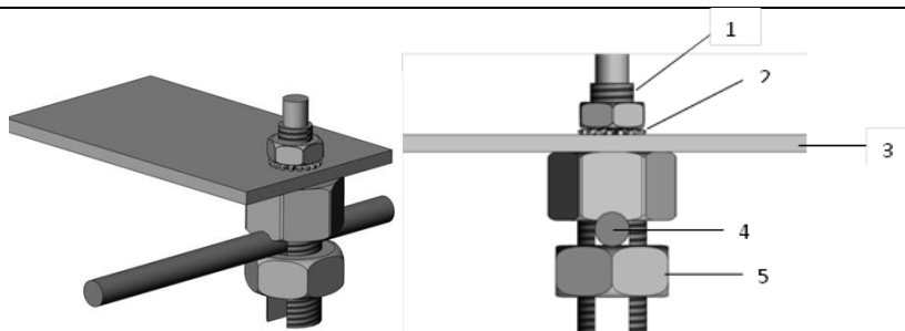
Figure 4. Tyco grounding bolt # 2058729-1
