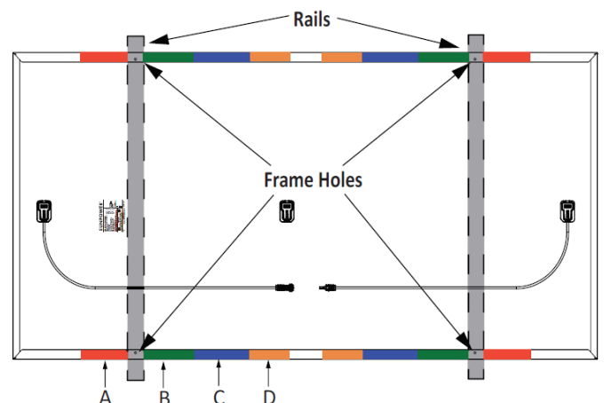
Figure 4: Mounting Zone Locations for Performance modules
