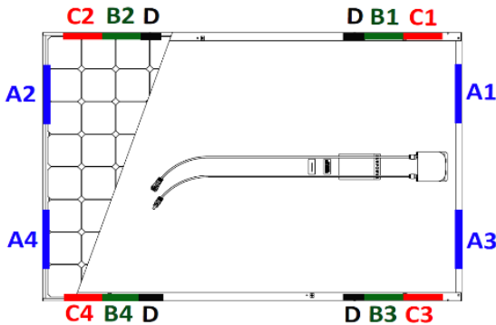
Figure 2: Mounting Zone locations for SunPower modules
