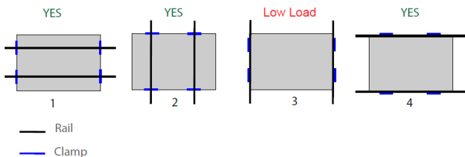
Figure 3: Mounting Configurations
